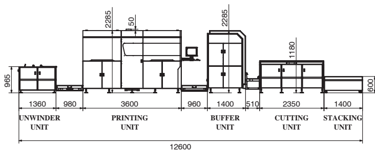
ROLL TO SHEET (ZIG-ZAG STACKING)
