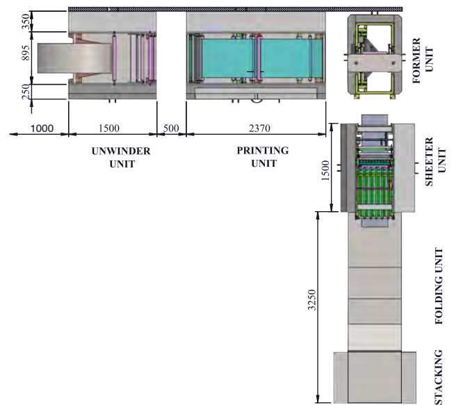
ROLL TO FOLD
